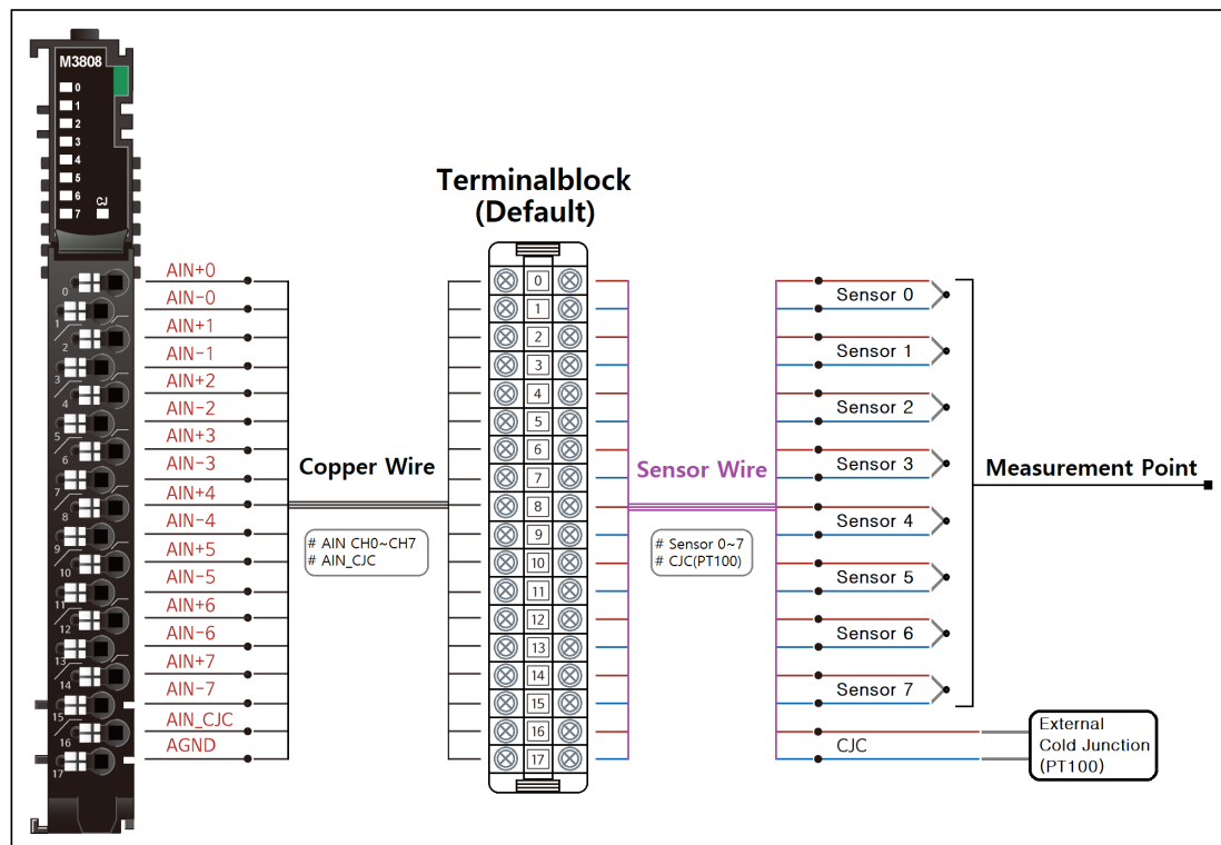
Configuration with cold junction (default)
