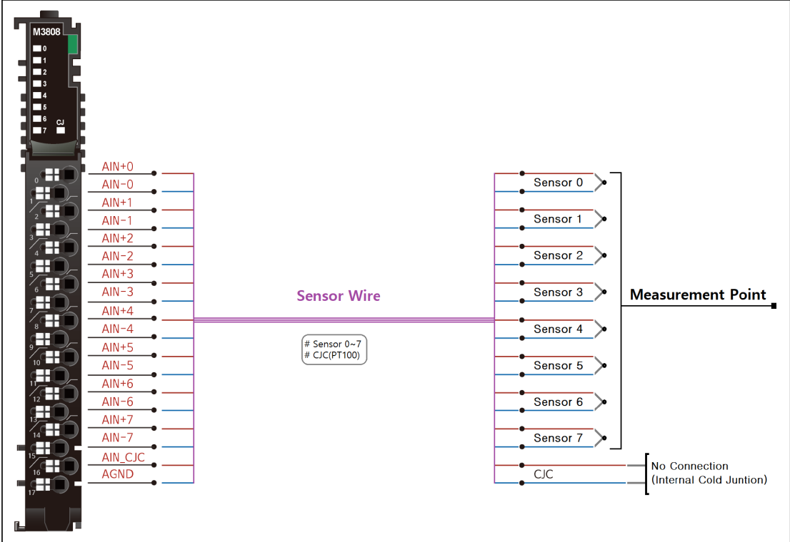
Configuration without cold junction
