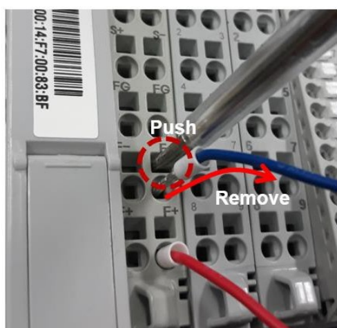
Disconnect cable
